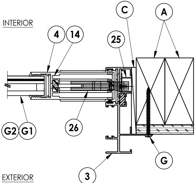
2 2 HORIZONTAL CROSS SECTION 2X Stud Construction
