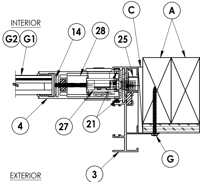
3 2 HORIZONTAL CROSS SECTION 2X Stud Construction
